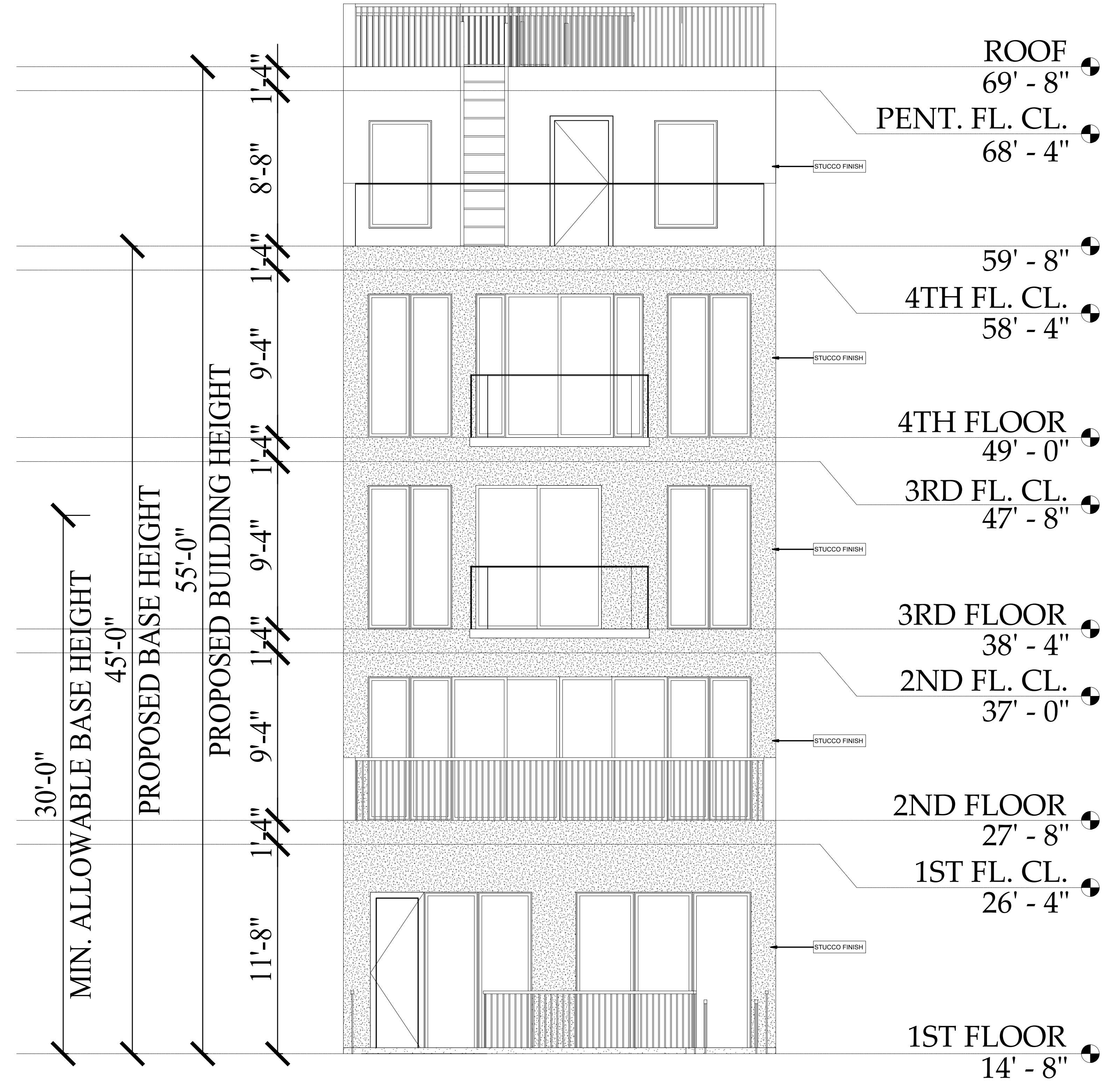
BACK ELEVATION (NORTH)
