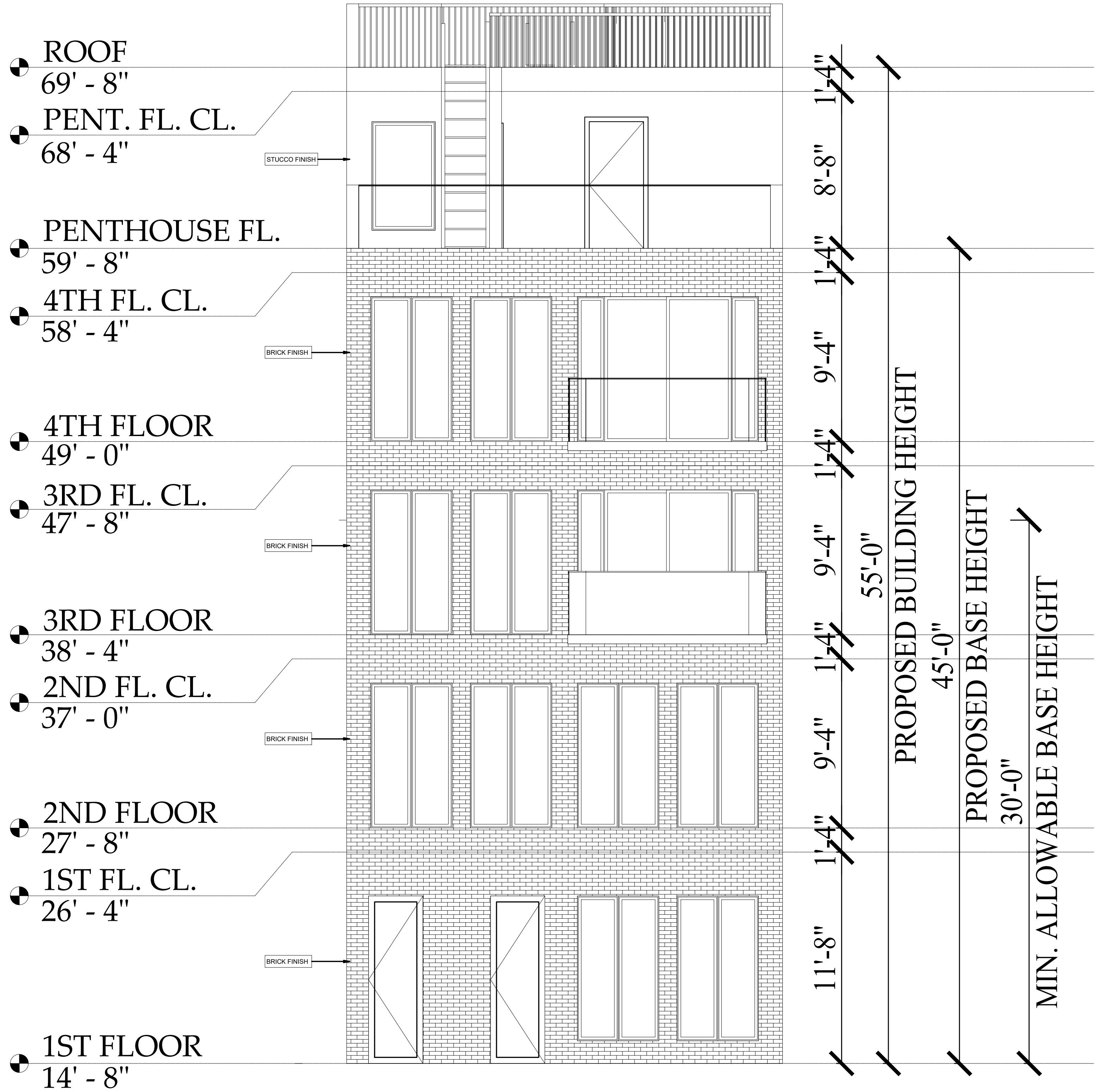
FRONT ELEVATION (SOUTH)
