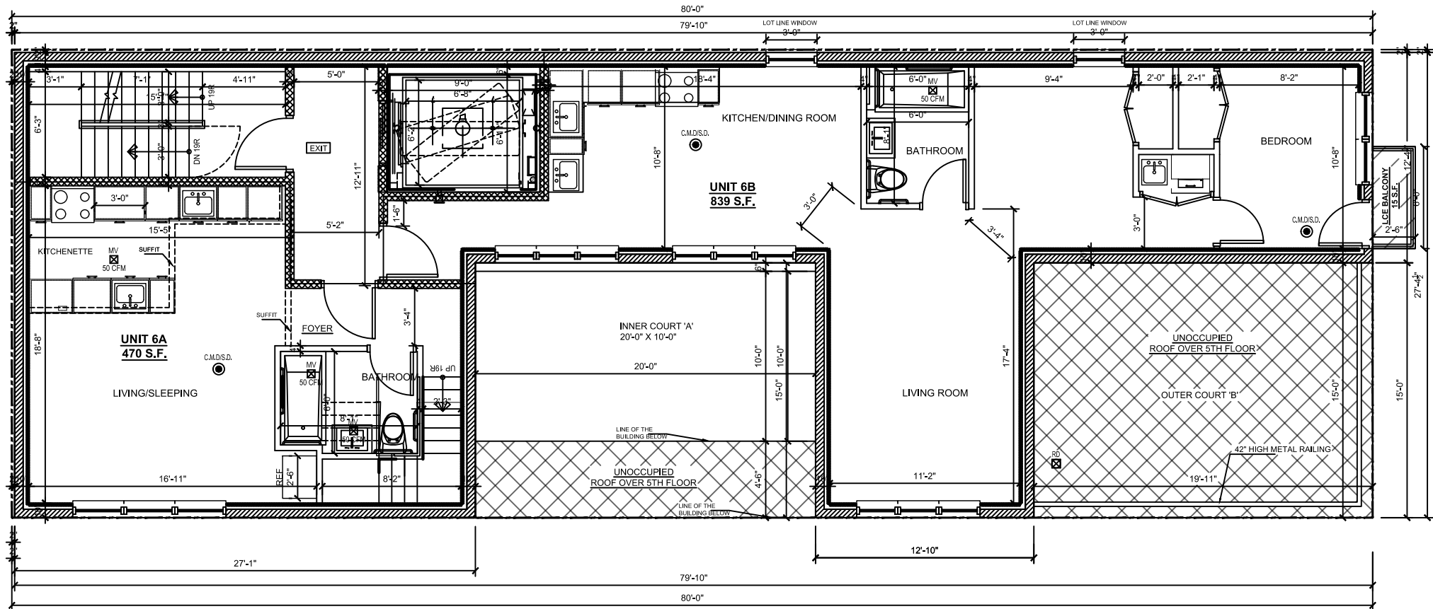
SIXTH FLOOR PLAN
