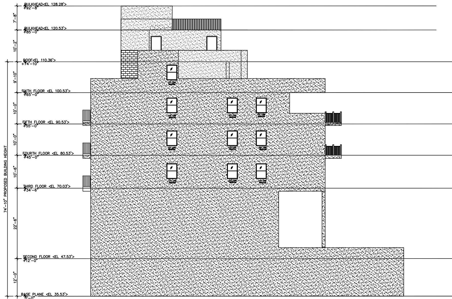
RIGHT HAND SIDE ELEVATION
