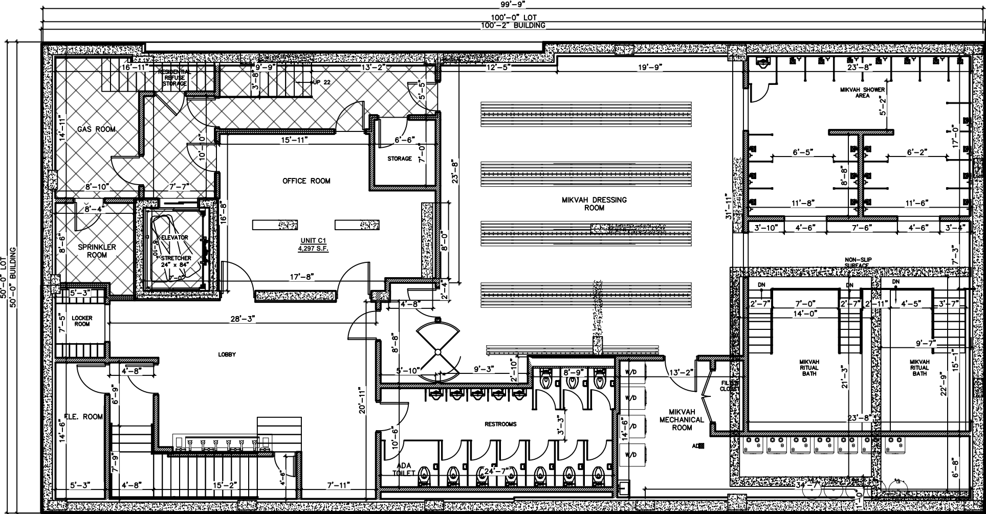
CELLAR FLOOR PLAN
