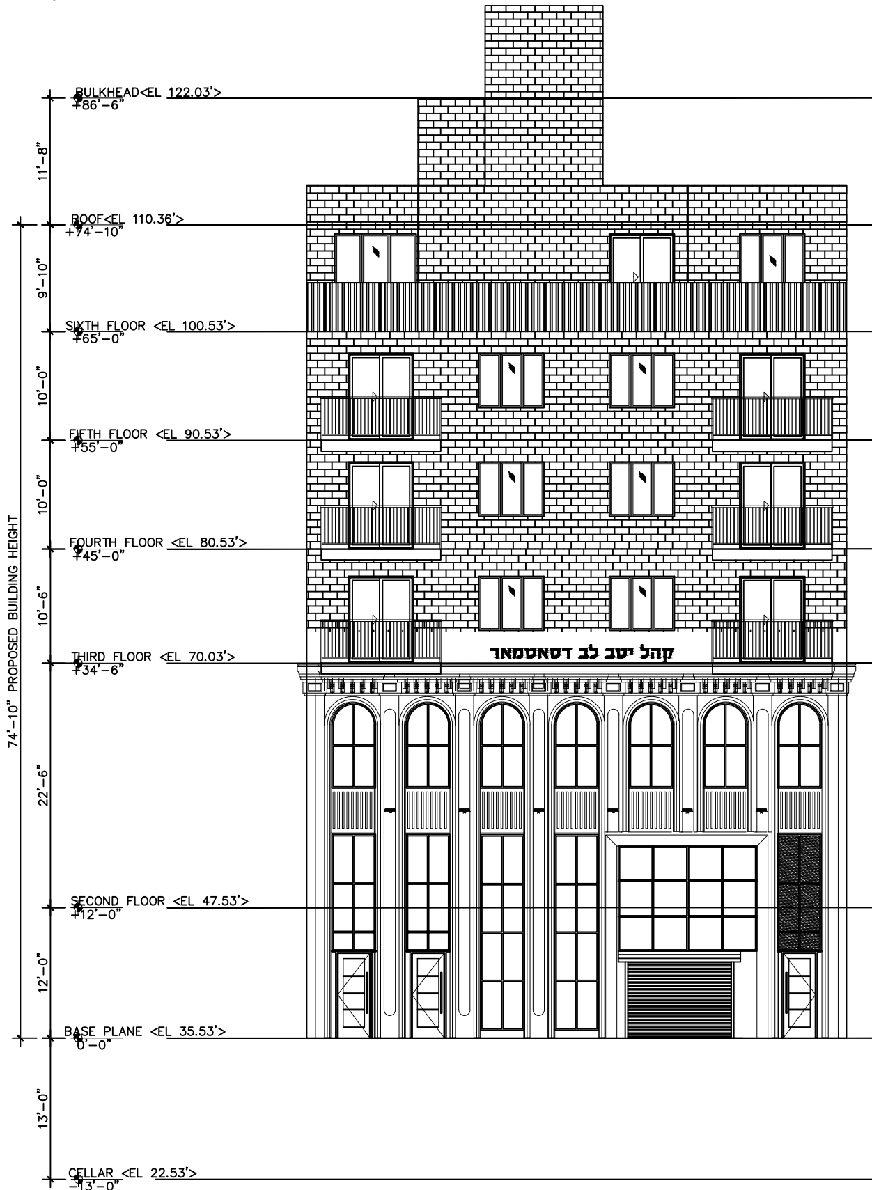
FRONT ELEVATION
