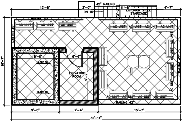
BULKHEAD FLOOR PLAN
