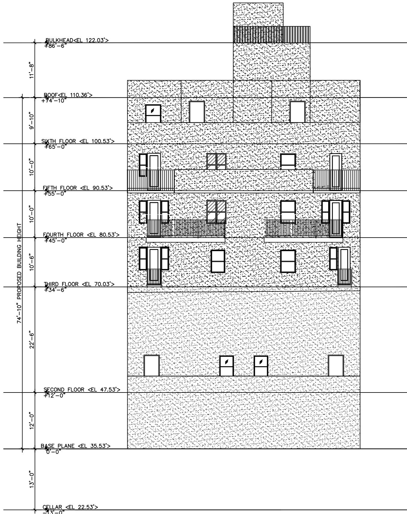
REAR ELEVATION
