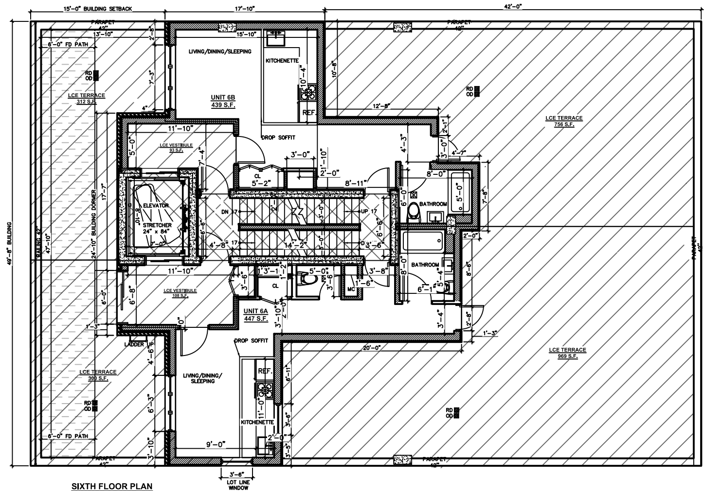
SIXTH FLOOR PLAN
